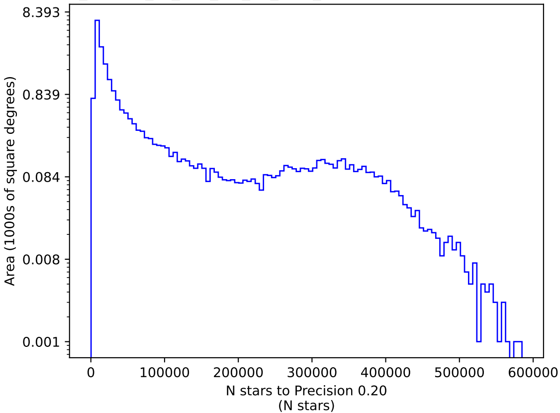
rolling_phased_ps_182_psf_91_v3.3_10yrs y: N stars to Precision 0.20
