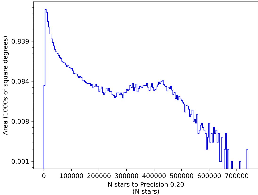
rolling_phased_ps_182_psf_91_v3.3_10yrs r: N stars to Precision 0.20
