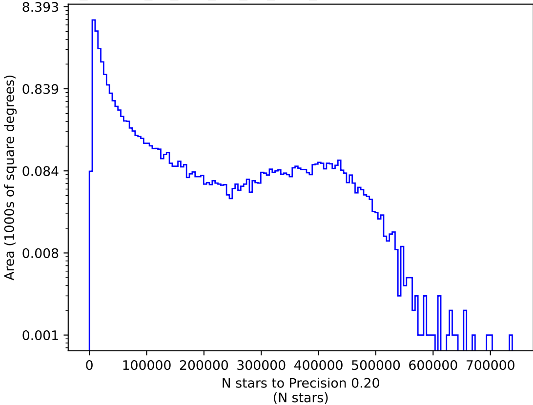
rolling_phased_ps_182_psf_91_v3.3_10yrs i: N stars to Precision 0.20
