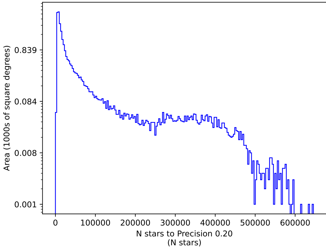
rolling_phased_ps_182_psf_91_v3.3_10yrs g: N stars to Precision 0.20
