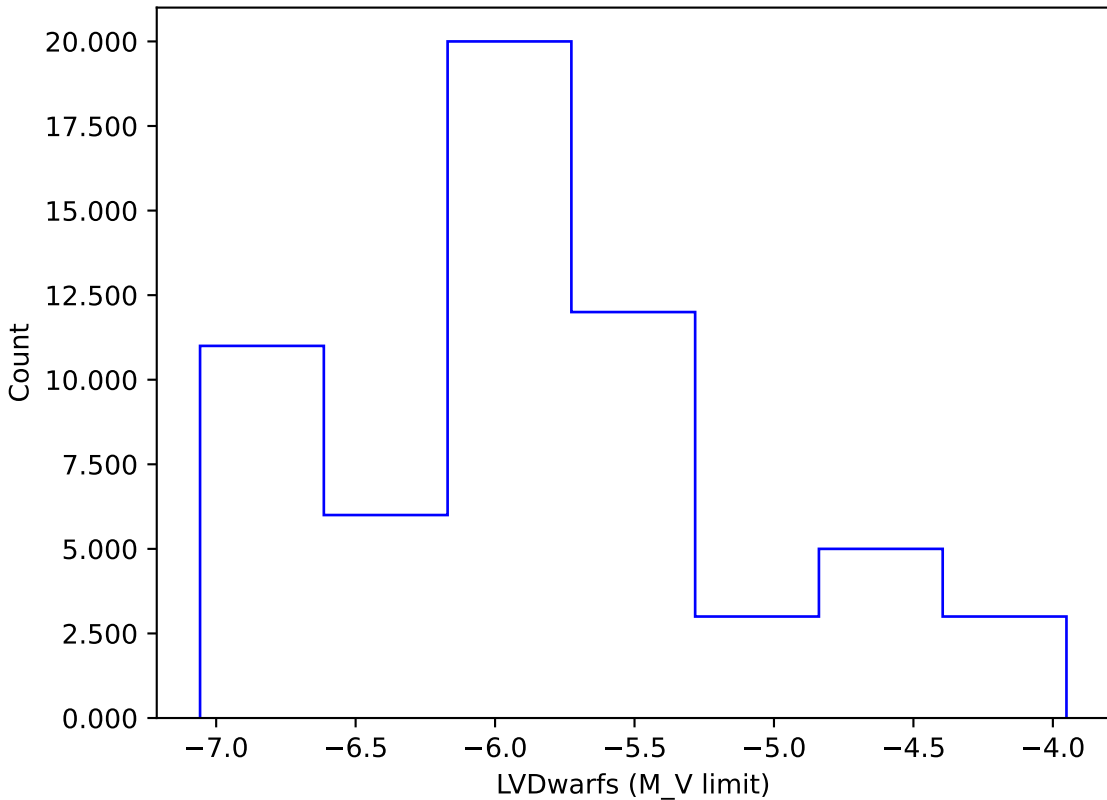
rolling_phased_ps_182_psf_91_v3.3_10yrs gi: LVDwarfs
