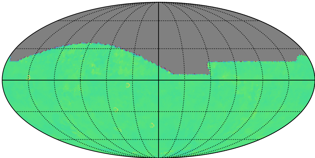
rolling_phased_ps_182_psf_91_v3.3_10yrs z: Kuiper rotTelPos
