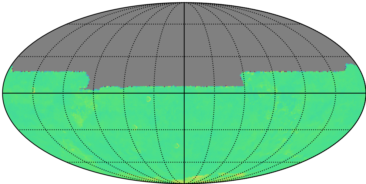
rolling_phased_ps_182_psf_91_v3.3_10yrs y: Kuiper rotTelPos
