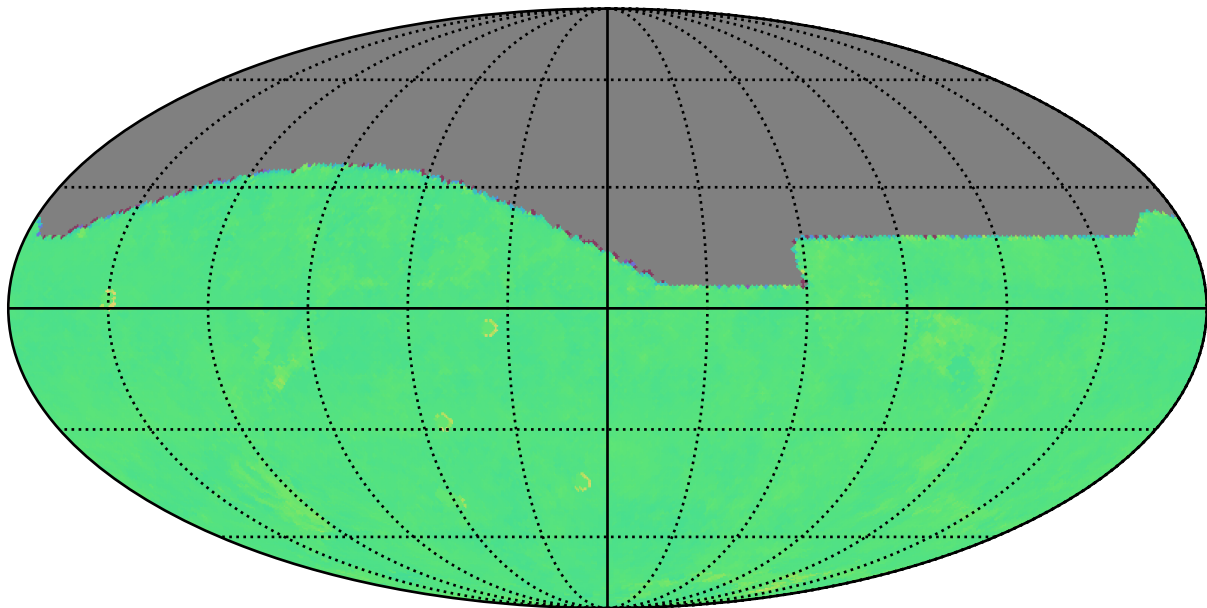
rolling_phased_ps_182_psf_91_v3.3_10yrs i: Kuiper rotTelPos
