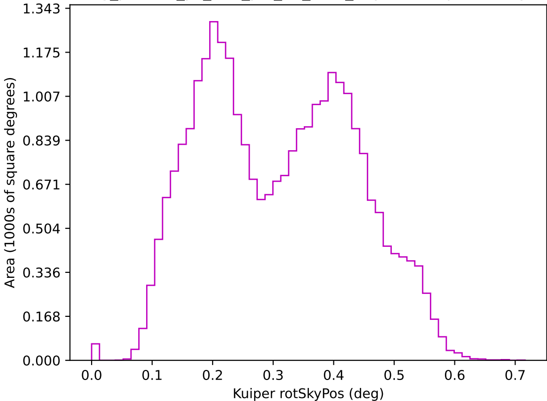
rolling_phased_ps_182_psf_91_v3.3_10yrs z: Kuiper rotSkyPos
