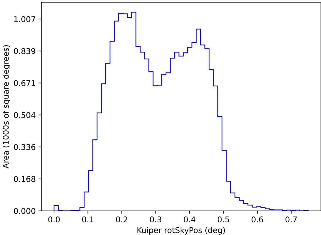
rolling_phased_ps_182_psf_91_v3.3_10yrs y: Kuiper rotSkyPos
