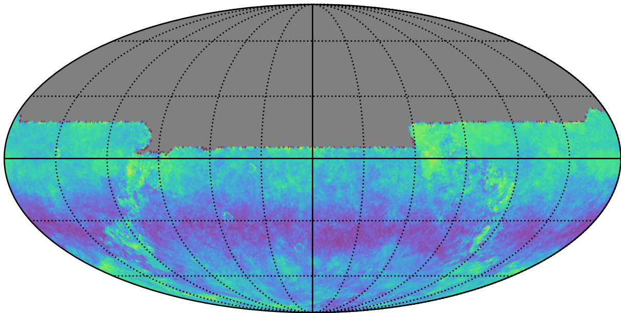
rolling_phased_ps_182_psf_91_v3.3_10yrs u: Kuiper rotSkyPos
