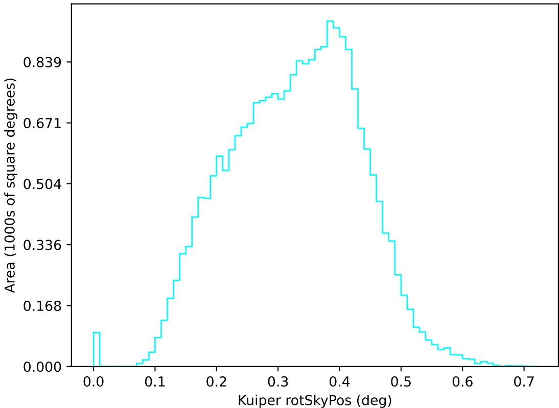
rolling_phased_ps_182_psf_91_v3.3_10yrs u: Kuiper rotSkyPos
