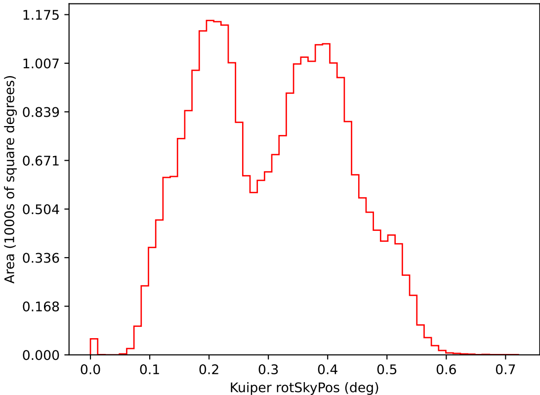
rolling_phased_ps_182_psf_91_v3.3_10yrs i: Kuiper rotSkyPos
