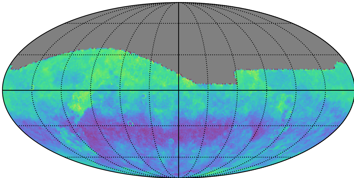
rolling_phased_ps_182_psf_91_v3.3_10yrs g: Kuiper rotSkyPos
