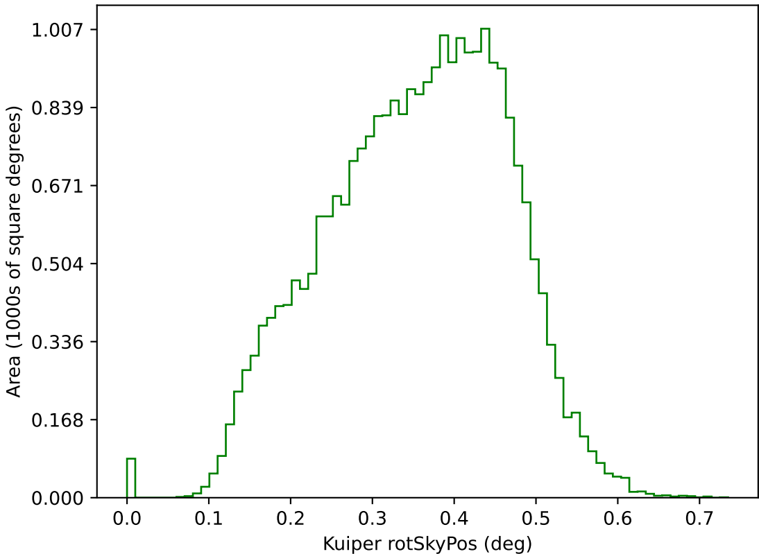
rolling_phased_ps_182_psf_91_v3.3_10yrs g: Kuiper rotSkyPos
