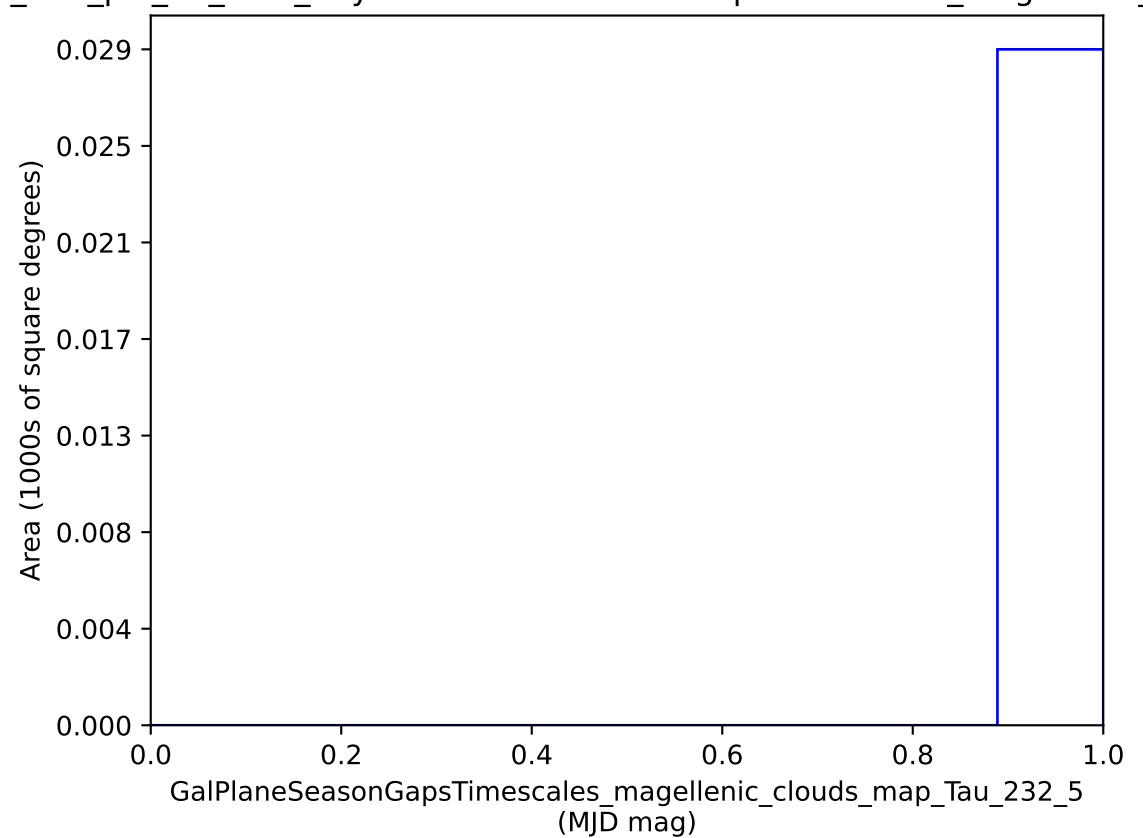
rolling_phased_ps_182_psf_91_v3.3_10yrs : GalPlaneSeasonGapsTimescales_magellenic_clouds_map_Tau_232_5
