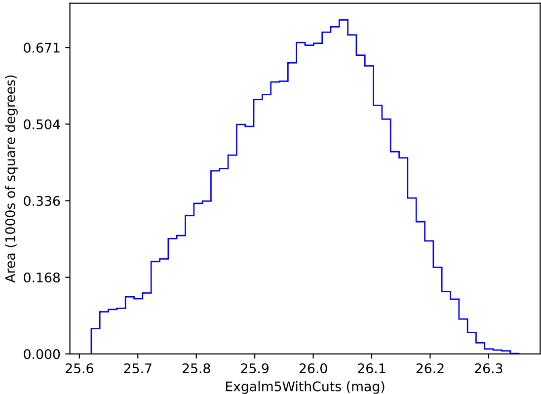
rolling_phased_ps_182_psf_91_v3.3_10yrs i band non-DD year 6: ExgalM5WithCuts
