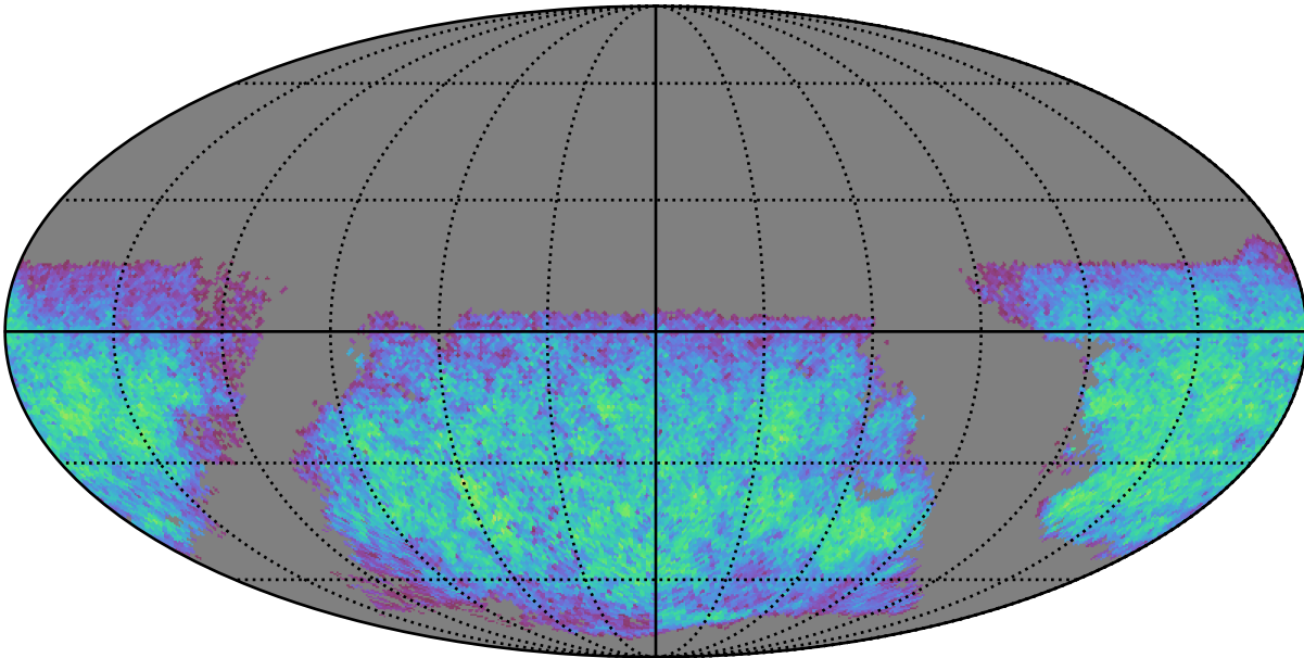
rolling_phased_ps_182_psf_91_v3.3_10yrs i band non-DD year 1: ExgalM5WithCuts
