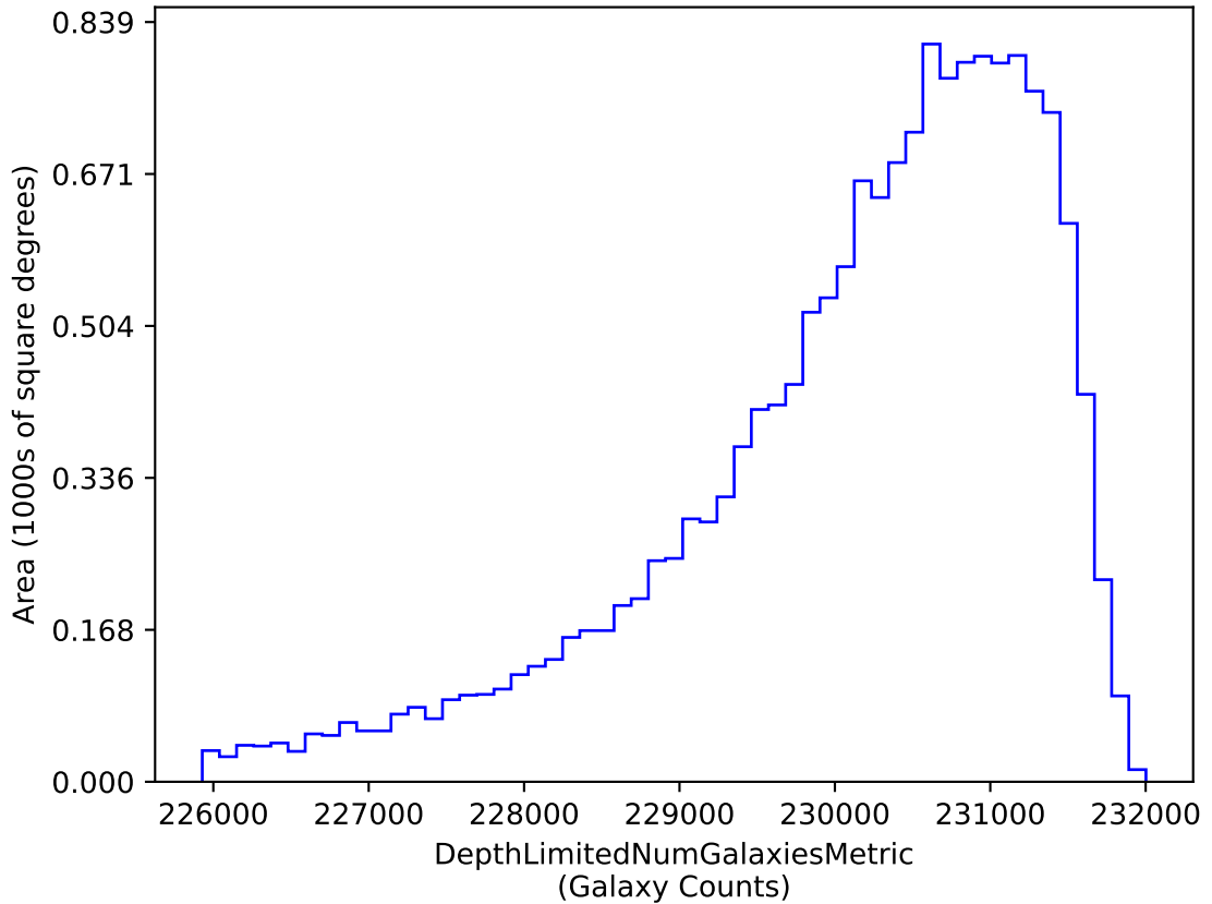
rolling_phased_ps_182_psf_91_v3.3_10yrs i band galaxies non-DD: DepthLimitedNumGalaxiesMetric
