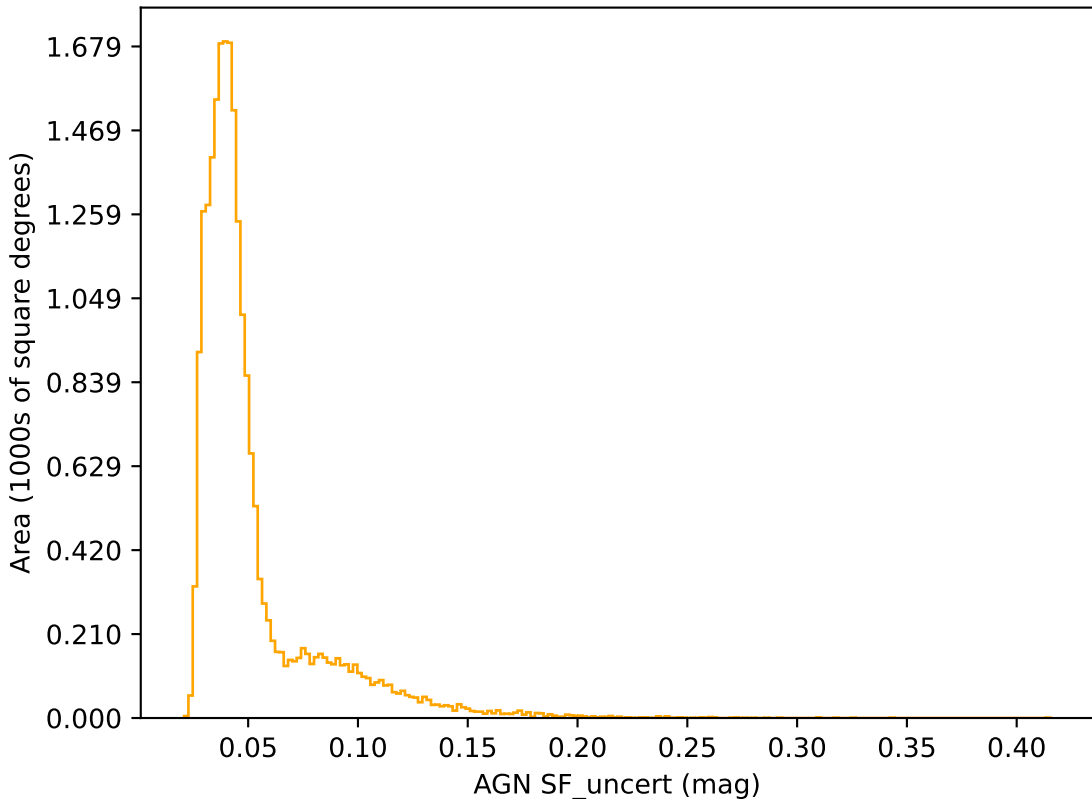
rolling_phased_ps_182_psf_91_v3.3_10yrs r band: AGN SF_uncert
