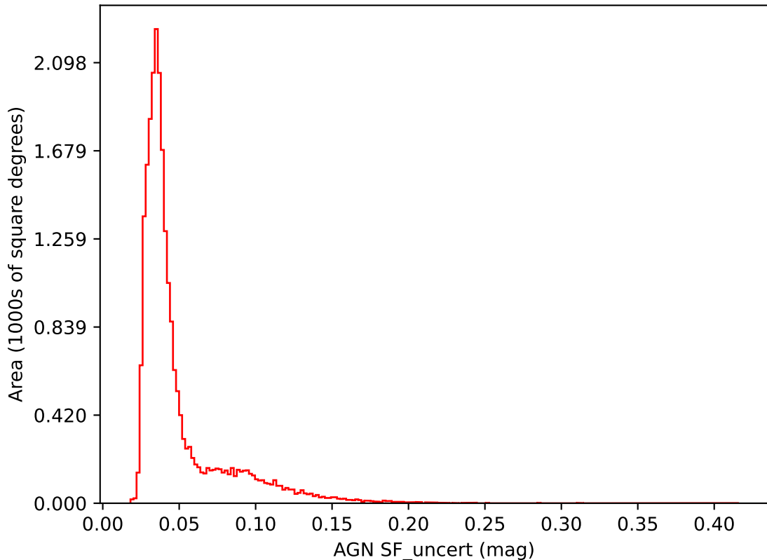
rolling_phased_ps_182_psf_91_v3.3_10yrs i band: AGN SF_uncert
