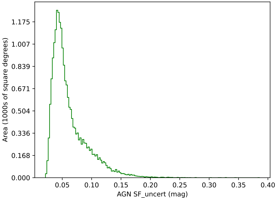
rolling_phased_ps_182_psf_91_v3.3_10yrs g band: AGN SF_uncert
