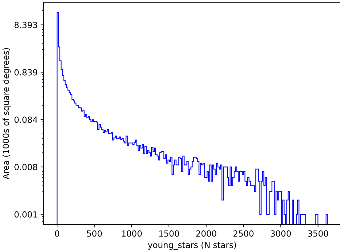
rolling_phased_ps_0_psf_0_v3.3_10yrs : young_stars
