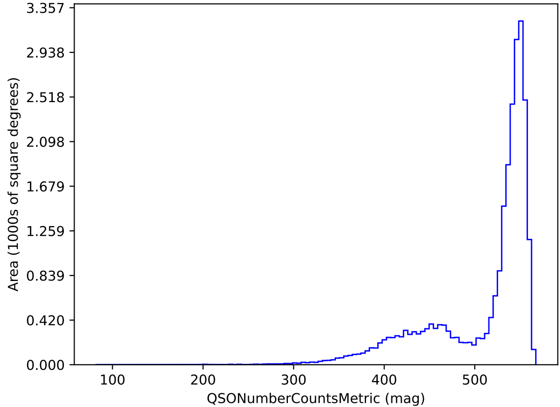
rolling_phased_ps_0_psf_0_v3.3_10yrs i band and non-DD: QSONumberCountsMetric
