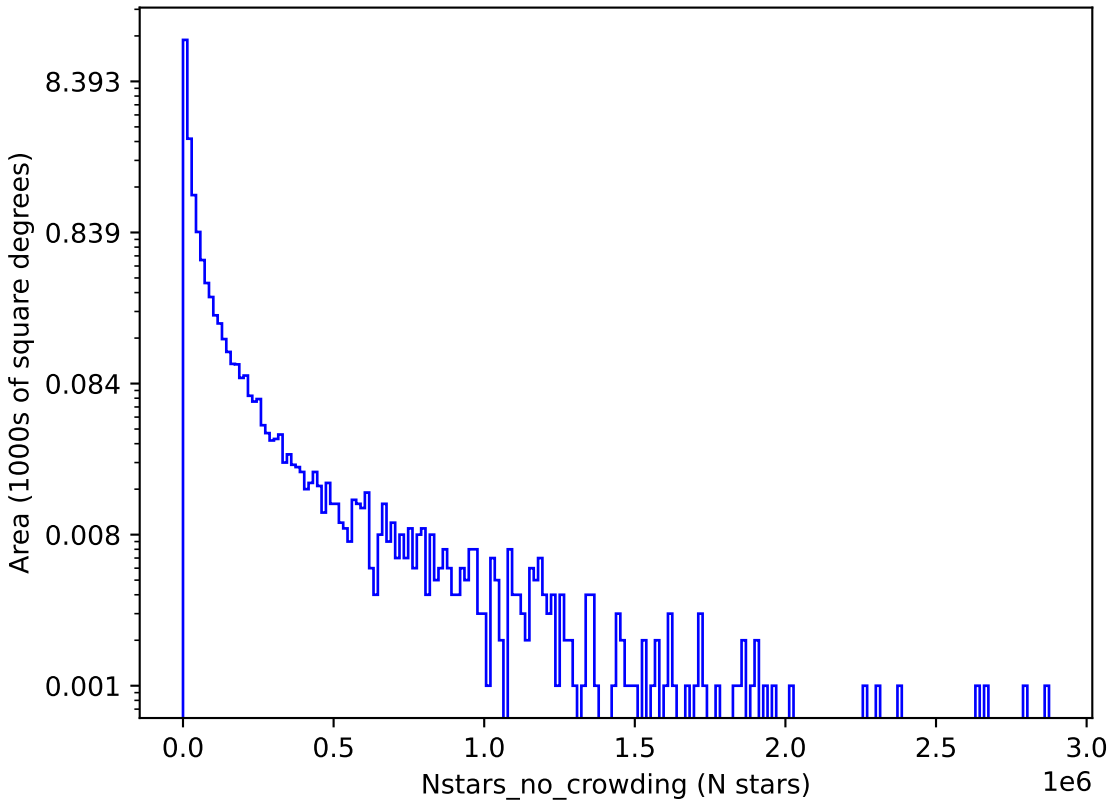
rolling_phased_ps_0_psf_0_v3.3_10yrs u: Nstars_no_crowding
