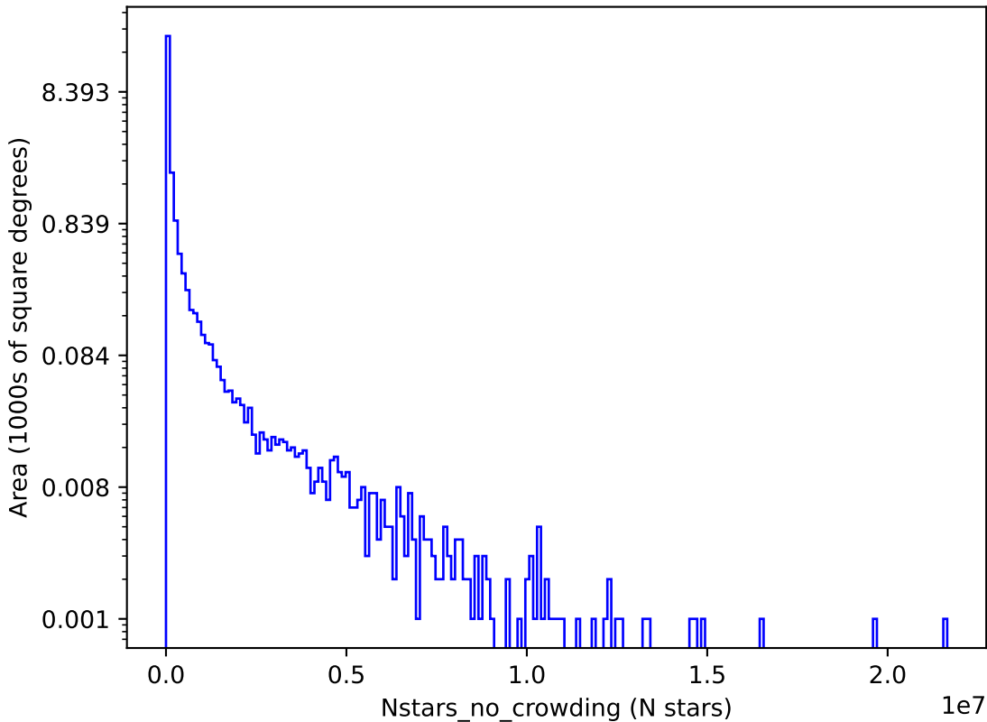
rolling_phased_ps_0_psf_0_v3.3_10yrs r: Nstars_no_crowding
