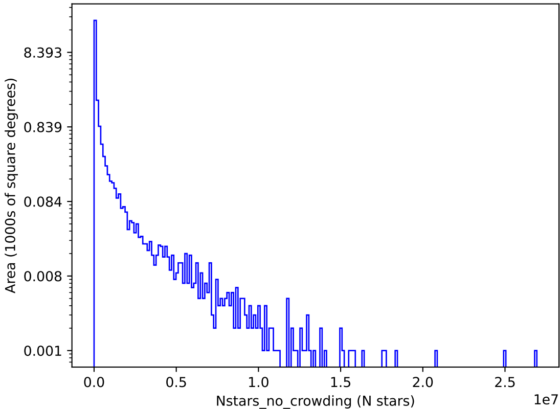
rolling_phased_ps_0_psf_0_v3.3_10yrs i: Nstars_no_crowding
