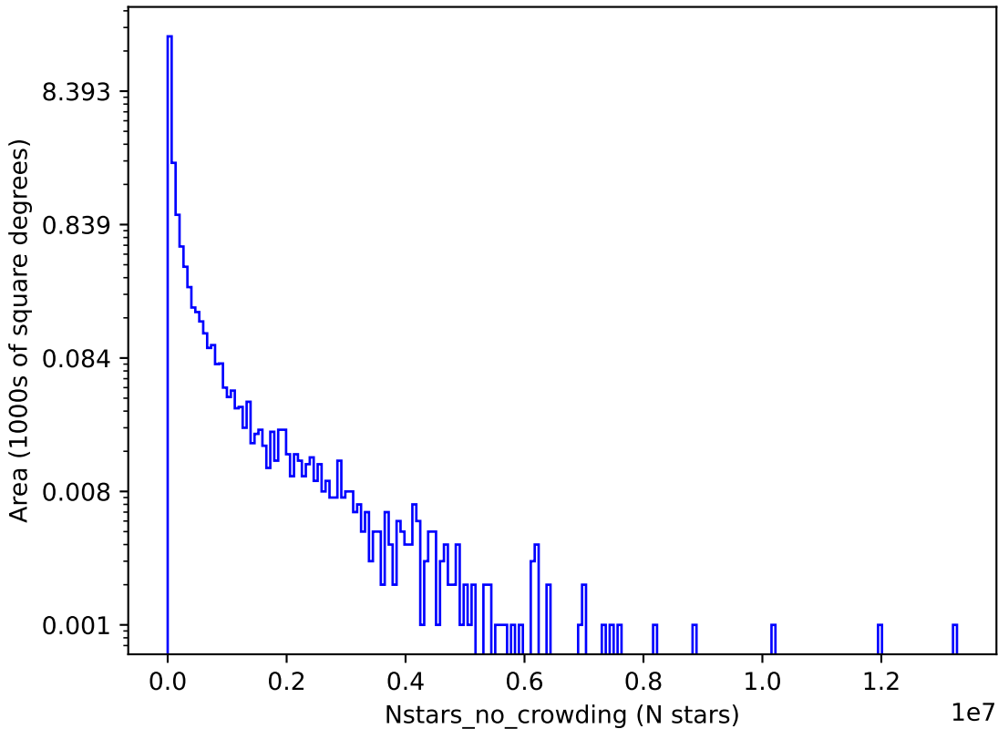
rolling_phased_ps_0_psf_0_v3.3_10yrs g: Nstars_no_crowding
