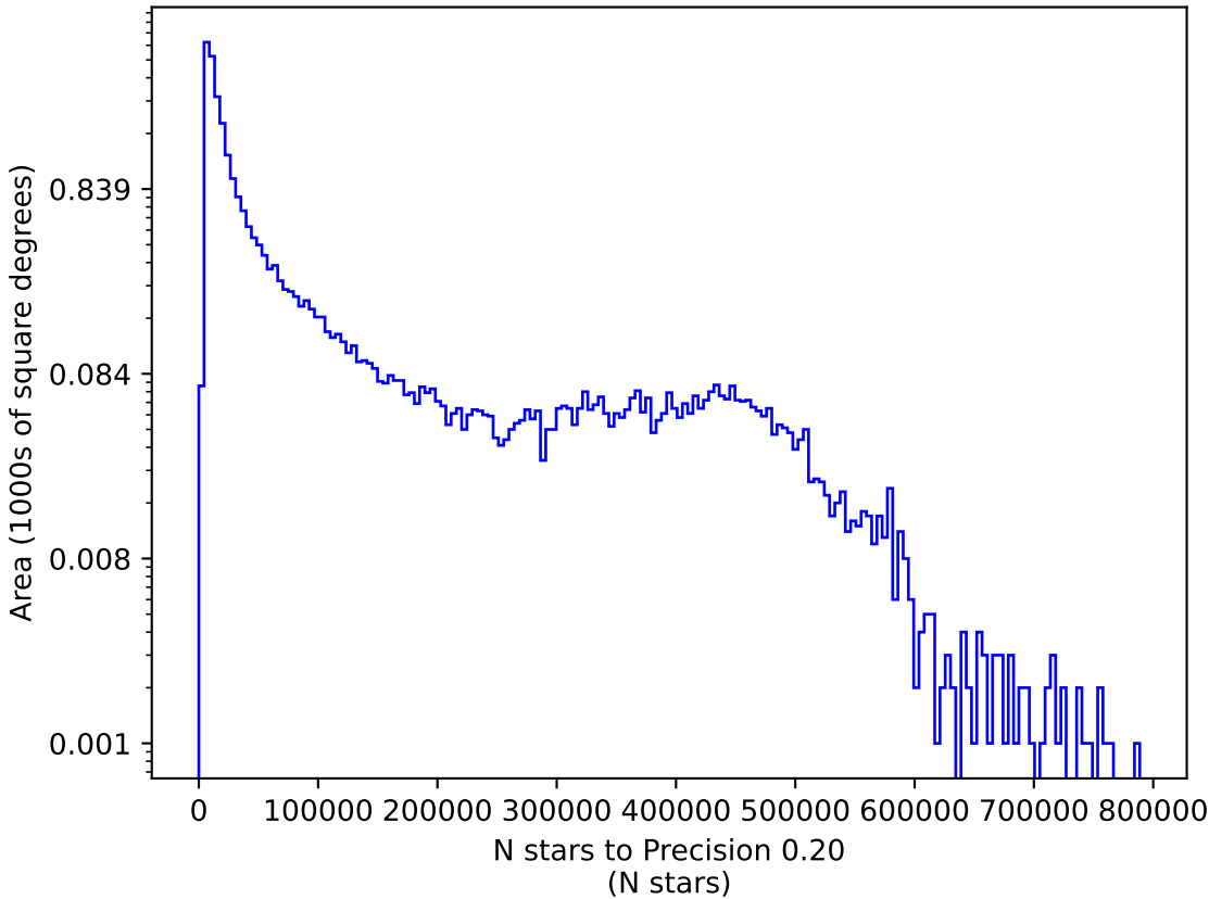
rolling_phased_ps_0_psf_0_v3.3_10yrs r: N stars to Precision 0.20
