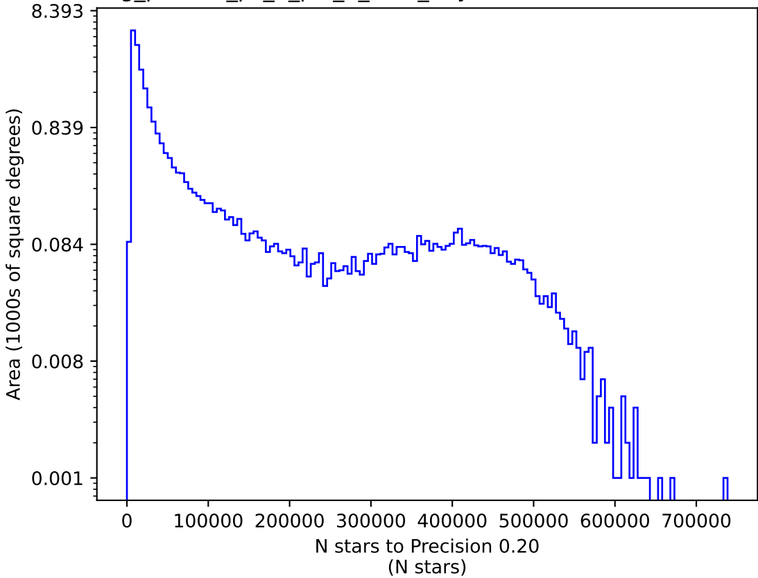
rolling_phased_ps_0_psf_0_v3.3_10yrs i: N stars to Precision 0.20
