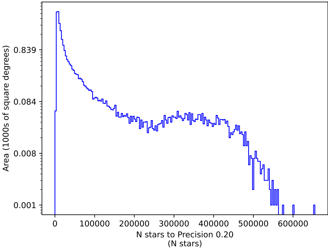
rolling_phased_ps_0_psf_0_v3.3_10yrs g: N stars to Precision 0.20
