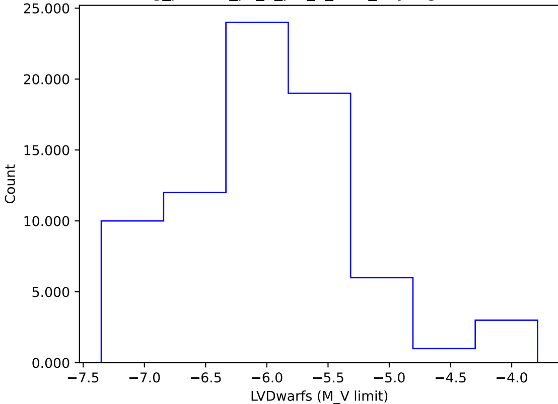
rolling_phased_ps_0_psf_0_v3.3_10yrs gi: LVDwarfs
