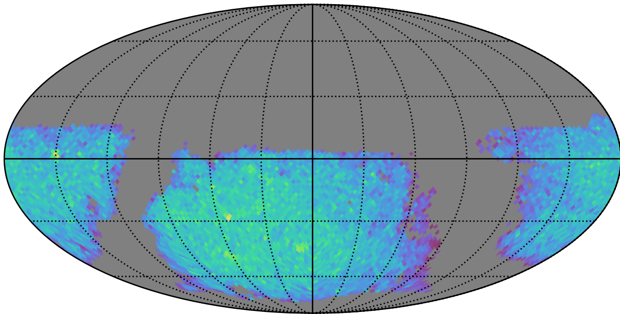
rolling_phased_ps_0_psf_0_v3.3_10yrs gi: LVDwarfs
