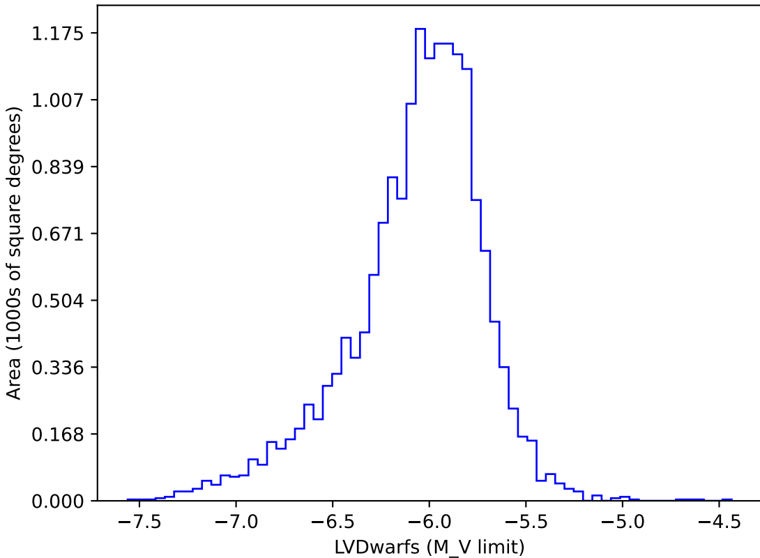
rolling_phased_ps_0_psf_0_v3.3_10yrs gi: LVDwarfs
