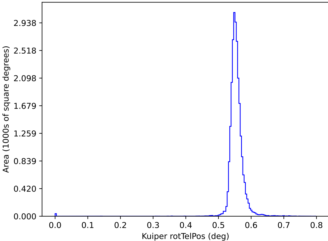
rolling_phased_ps_0_psf_0_v3.3_10yrs y: Kuiper rotTelPos
