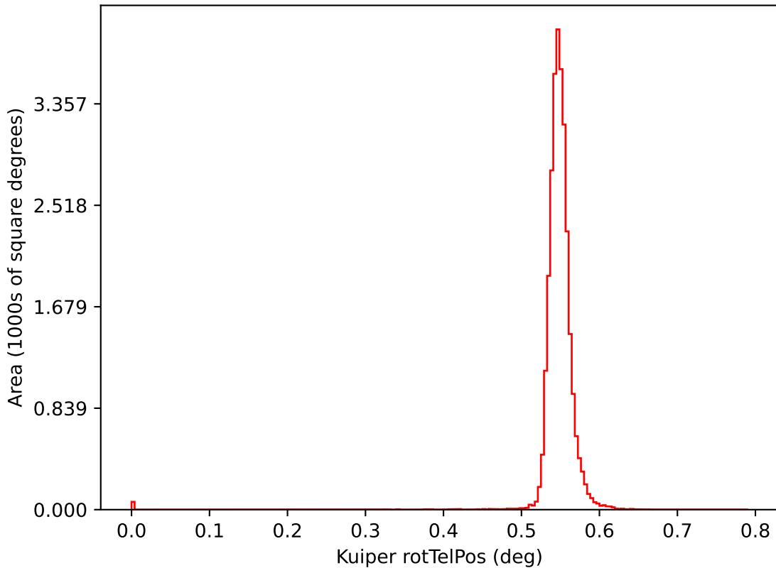
rolling_phased_ps_0_psf_0_v3.3_10yrs i: Kuiper rotTelPos
