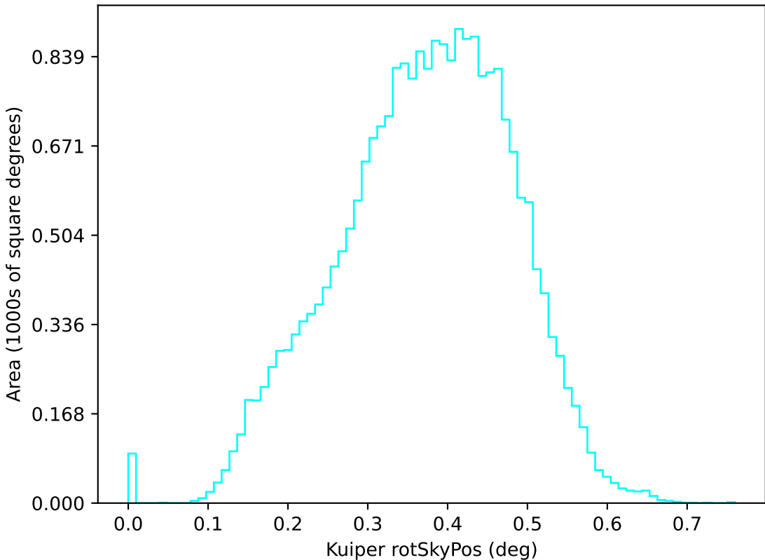
rolling_phased_ps_0_psf_0_v3.3_10yrs u: Kuiper rotSkyPos
