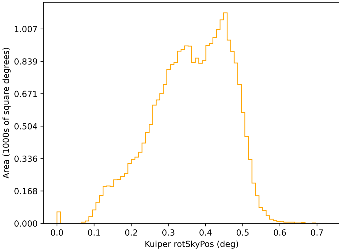
rolling_phased_ps_0_psf_0_v3.3_10yrs r: Kuiper rotSkyPos
