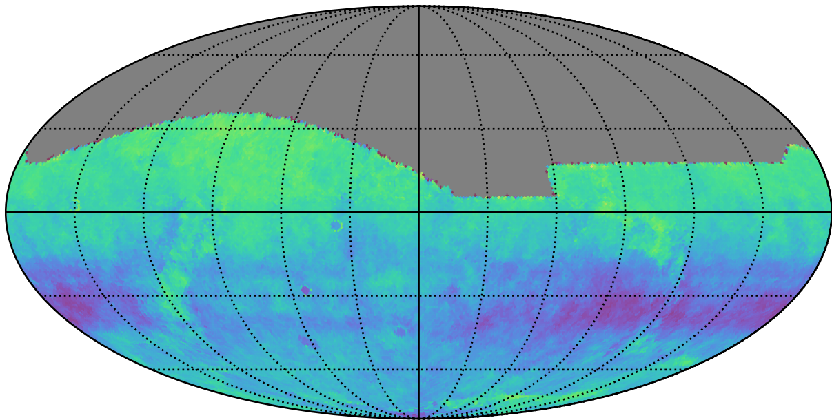
rolling_phased_ps_0_psf_0_v3.3_10yrs i: Kuiper rotSkyPos
