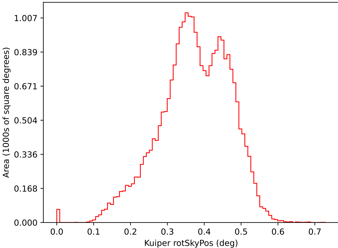
rolling_phased_ps_0_psf_0_v3.3_10yrs i: Kuiper rotSkyPos
