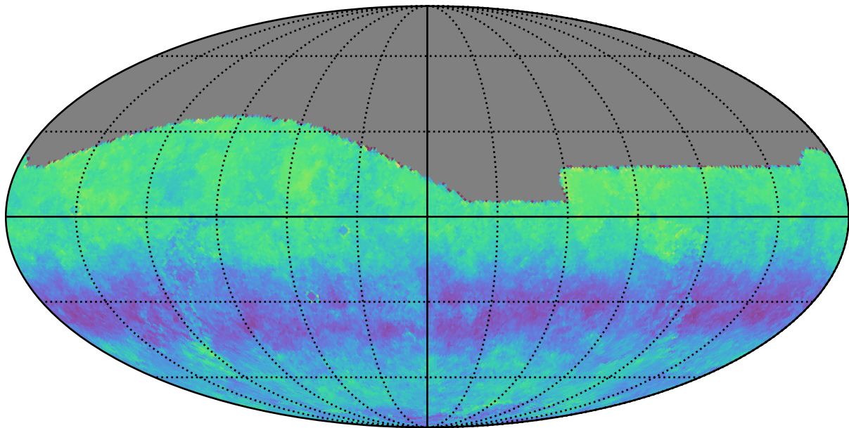
rolling_phased_ps_0_psf_0_v3.3_10yrs g: Kuiper rotSkyPos
