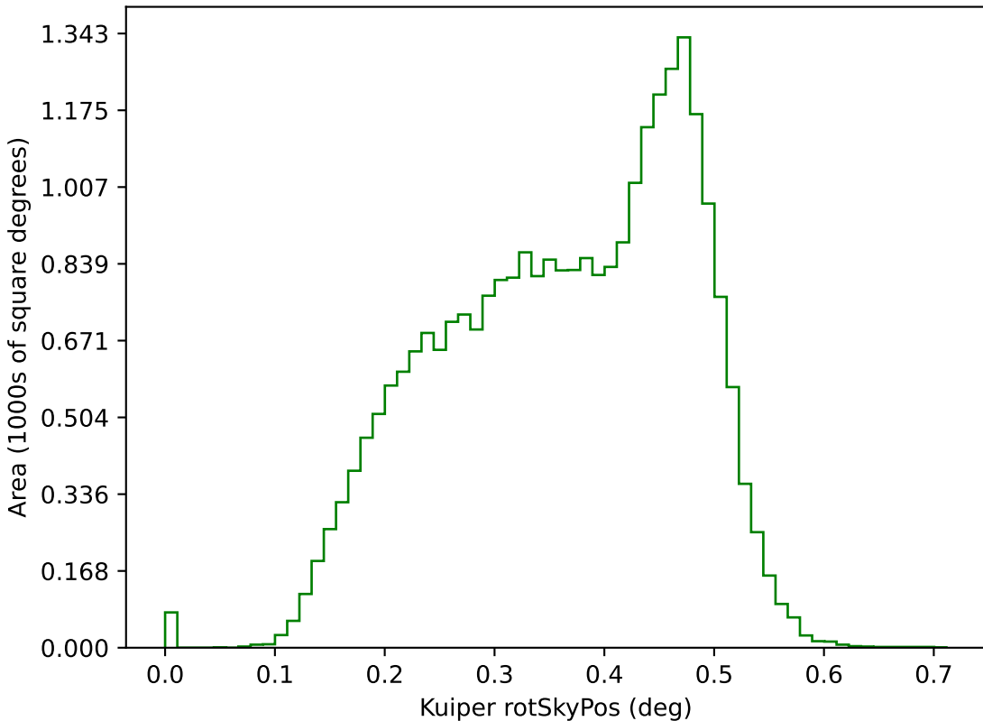
rolling_phased_ps_0_psf_0_v3.3_10yrs g: Kuiper rotSkyPos
