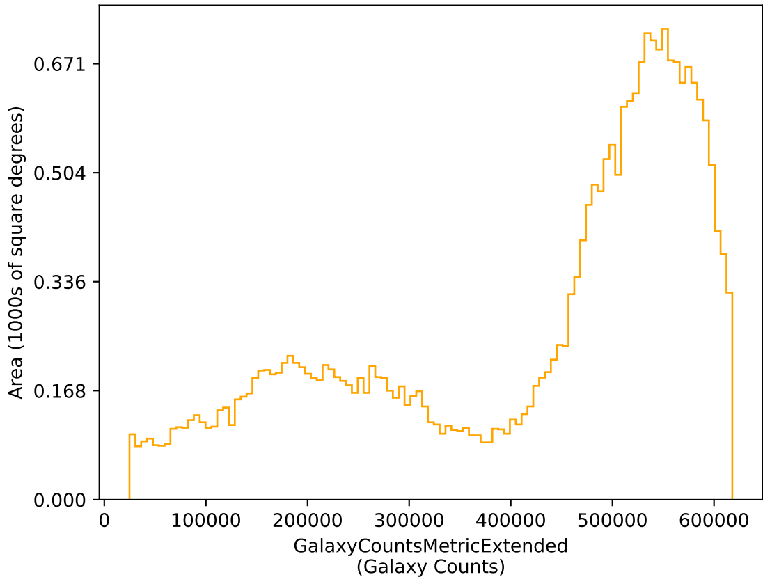
rolling_phased_ps_0_psf_0_v3.3_10yrs r: GalaxyCountsMetricExtended
