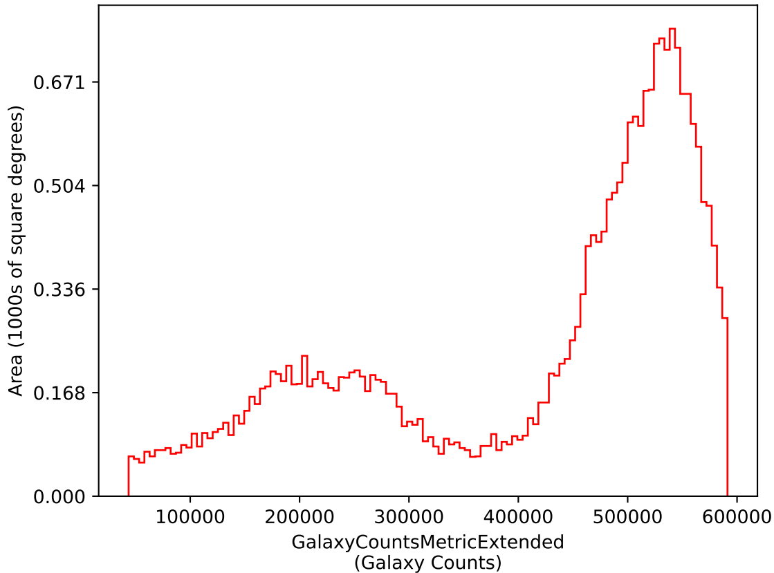
rolling_phased_ps_0_psf_0_v3.3_10yrs i: GalaxyCountsMetricExtended
