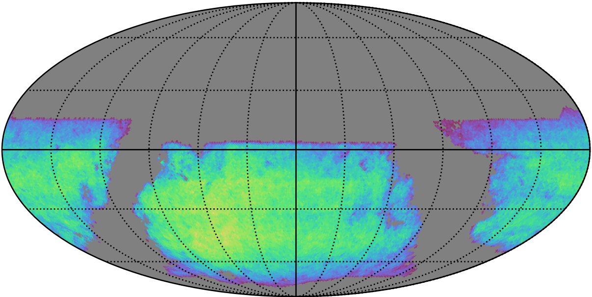
rolling_phased_ps_0_psf_0_v3.3_10yrs i band non-DD year 8: ExgalM5WithCuts
