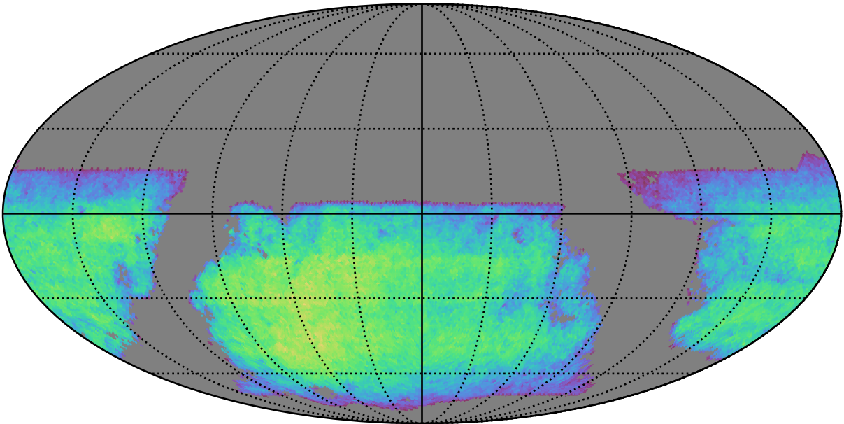
rolling_phased_ps_0_psf_0_v3.3_10yrs i band non-DD year 6: ExgalM5WithCuts
