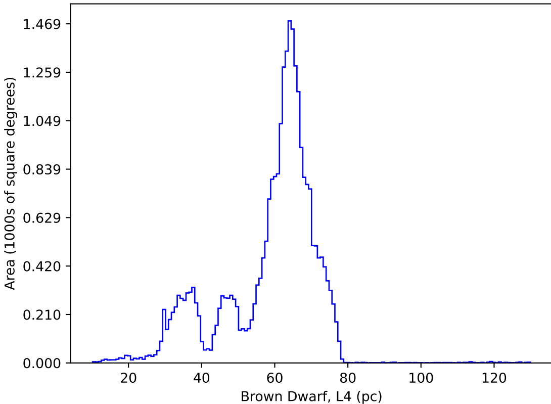
rolling_phased_ps_0_psf_0_v3.3_10yrs : Brown Dwarf, L4
