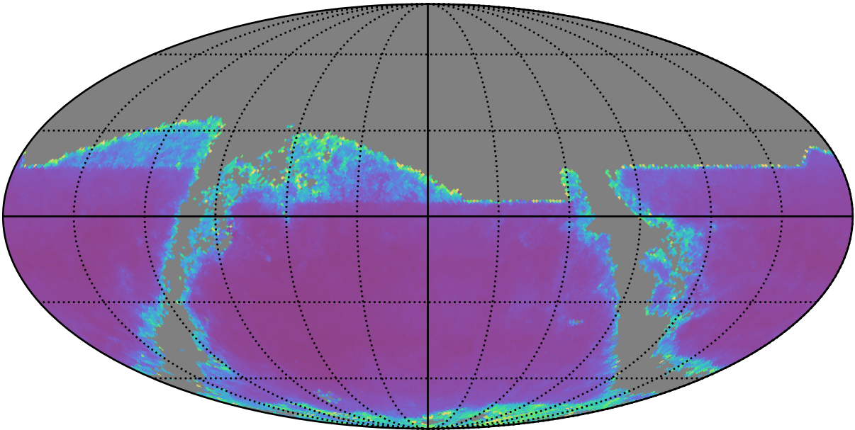
rolling_phased_ps_0_psf_0_v3.3_10yrs i band: AGN SF_uncert
