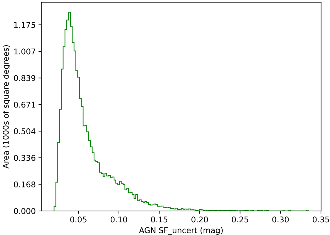
rolling_phased_ps_0_psf_0_v3.3_10yrs g band: AGN SF_uncert
