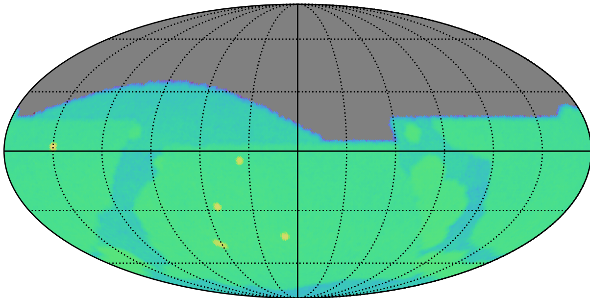
rolling_phased_ps_-182_psf_0_v3.3_10yrs g: SurfaceBrightLimit
